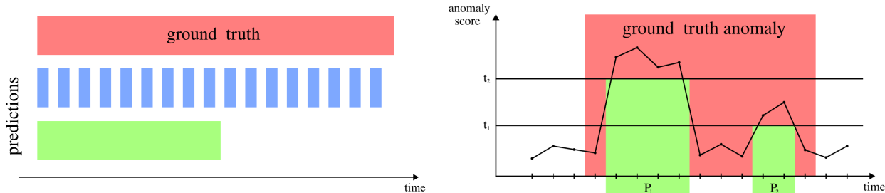
(a) Two predictions of equal size with distinct predictive patterns on an anomaly. (b) Anomaly score and predictions P_1, P_2 , where only the larger persists for both thresholds t_1, t_2 .
